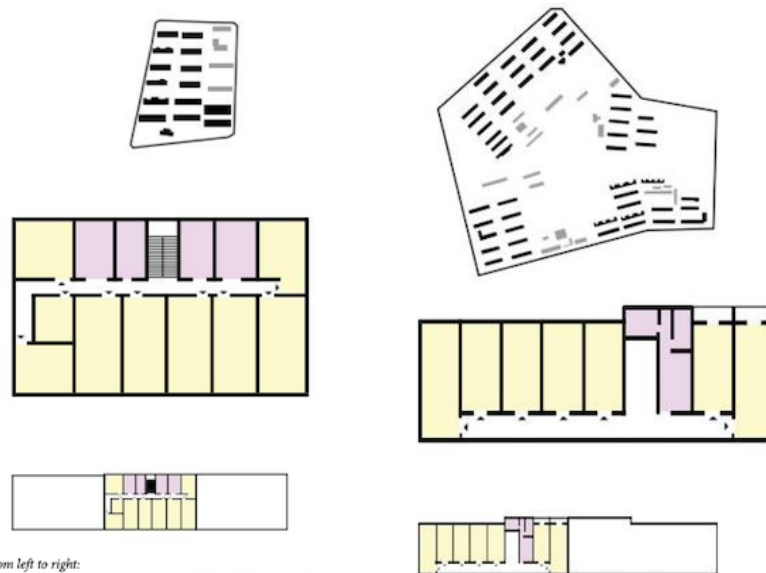
From left to right: Fig. 3.9 : The second generation of the KTT - KTT Nguyen Cong Tru (1963) (From top to bottom: 1- Site plan; 2 - Typical plan of an unit, 3 - Typical plan of a building [Credit: Author] Fig. 3.10 : The second generation of the KTT - KTT Kim Lien (1965) (From top to bottom: 1- Site plan; 2 - Typical plan of an unit; 3 - Typical plan of a building [Credit: Author]
